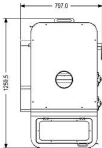
PLAN VIEW
