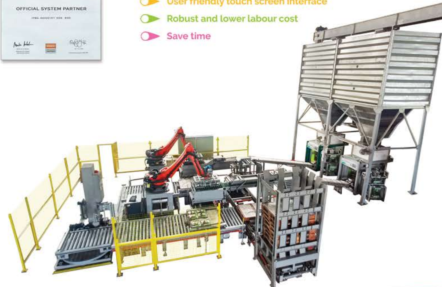
( 5 & 10kgs palletizing line )
