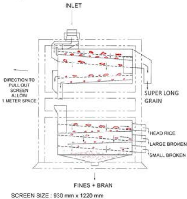
CONSTRUCTION & FLOW
